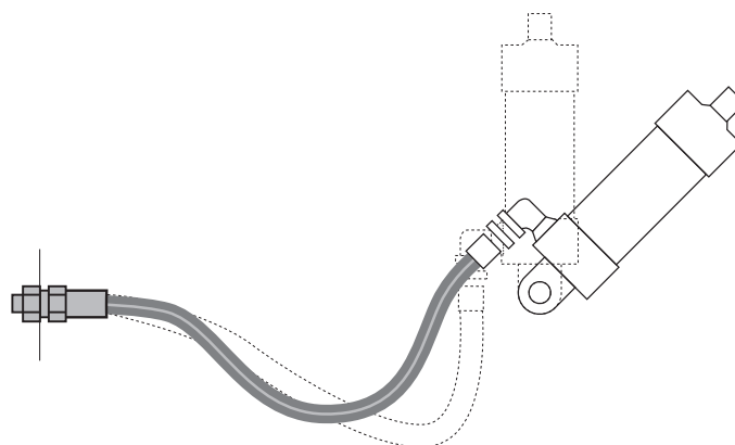
FIG. 4 MOTION ABSORPTION
