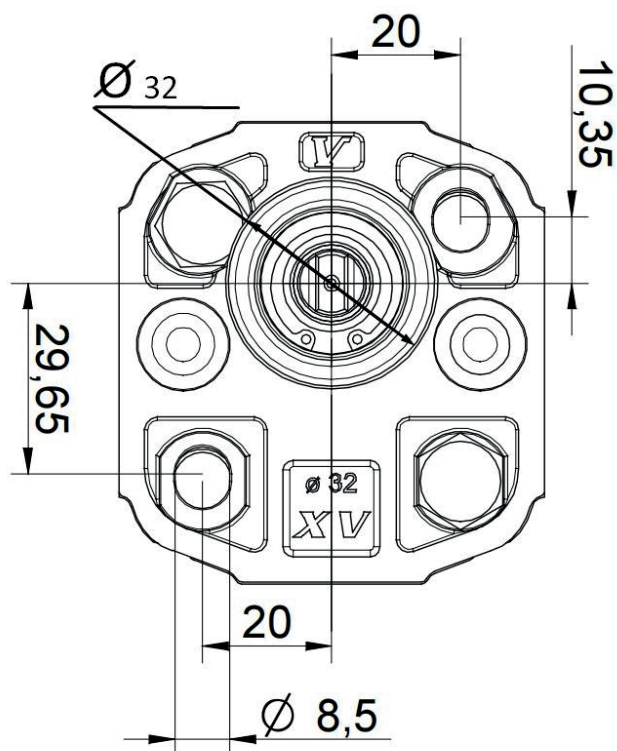
XV1 Ø32 BH-HY POMPA-FS (100.0271.AKP-FS)
