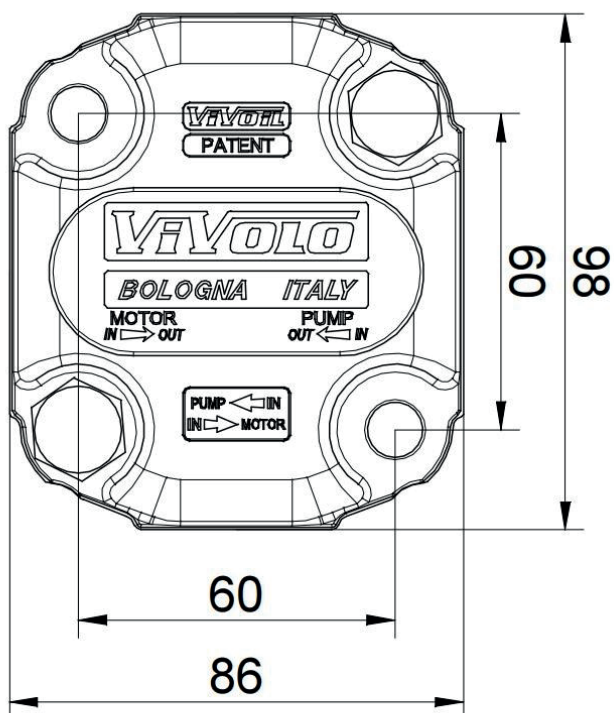
XV2 - P XV2 - U XV2 - F STANDARD (200.0237.AK)
