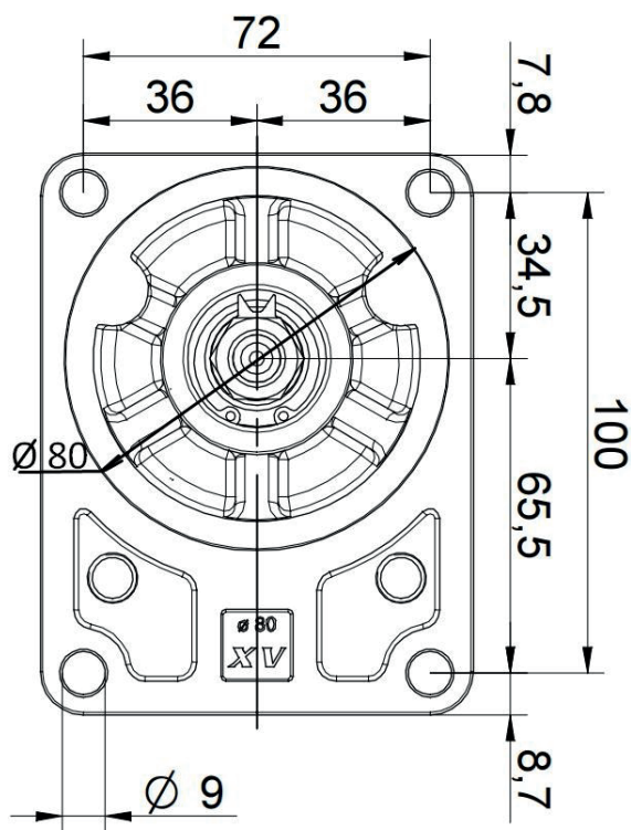
XV2 Ø80 (200.0239.AKP)
