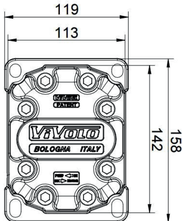
XV1-P XV1-U XV1-F STANDARD (100.0268.AK)
