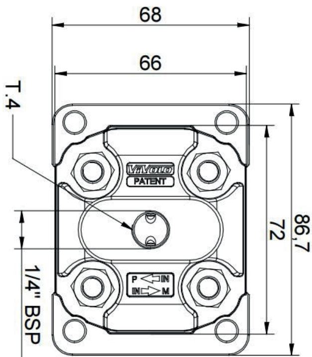
XV1-R XV1-M-DREN 1/4" BSP (100.0274.XK/F1ZZA)
