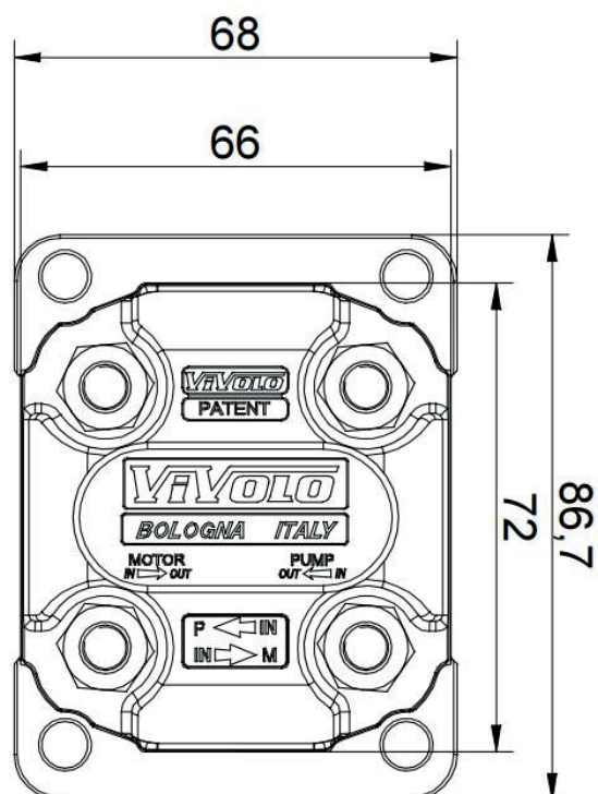
XV1-P XV1-U XV1-F STANDARD (100.0268.AK)
