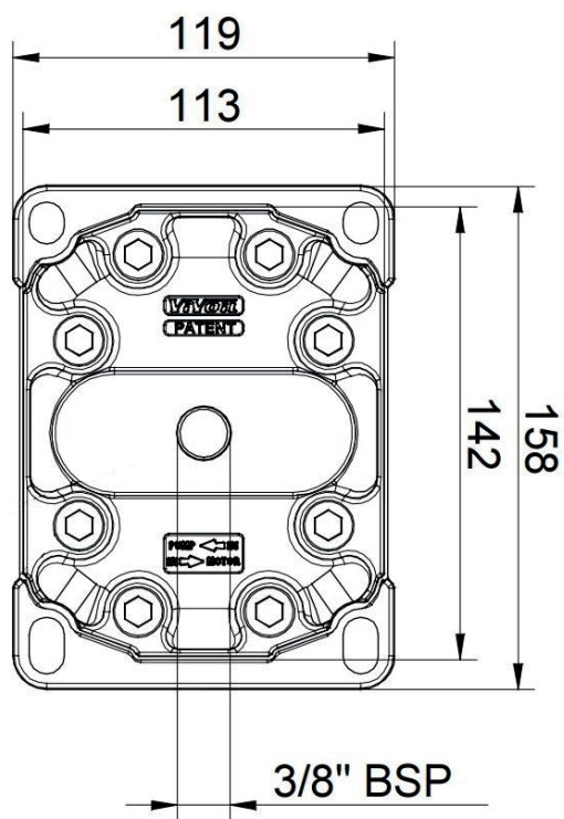
XV3R - DREN 3/8" (300.0134.XK - F3ZZL)
