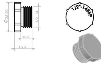
PVP04 Plastic Valve plug 1/2"
