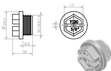
PVP18 Plastic Valve plug M18
