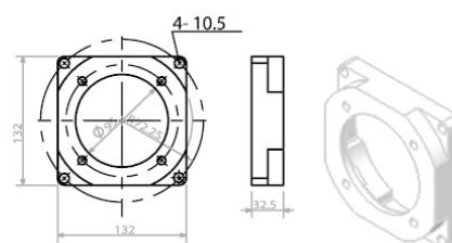
FMC90 90 Frame motor connector
