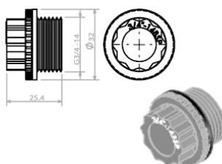
PVP06 Plastic Valve plug 3/4"
