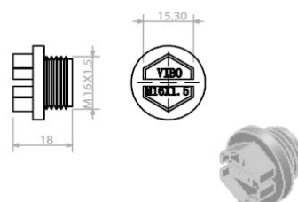
PVP16 Plastic Valve plug M16
