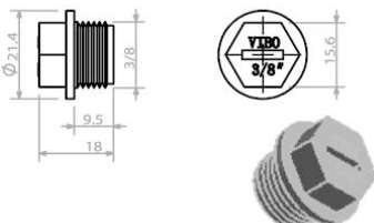
PVP03 Plastic Valve plug 3/8"
