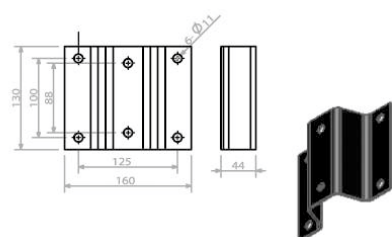
FM82 Mounting bracket
