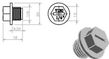
PVP02 Plastic Valve plug 1/4"
